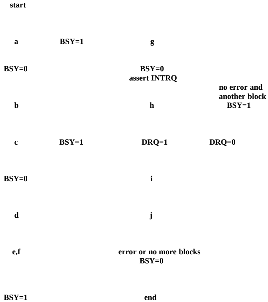
Figure 10 - PIO Data Transfer Diagram
